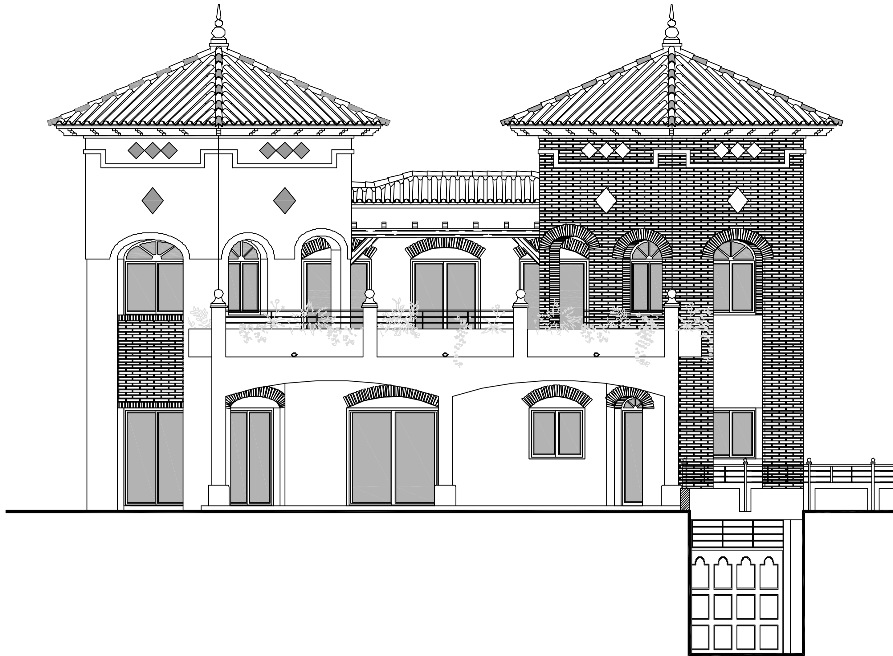
Alzado Principal
